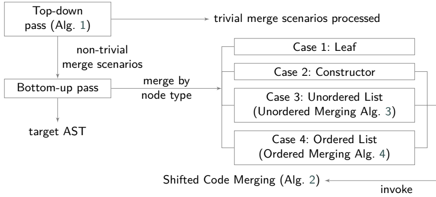
Figure 4: High-level workflow of our merge algorithm.
