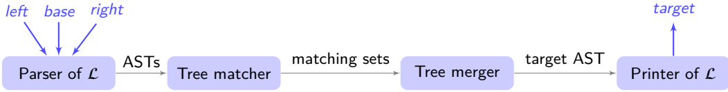
Figure 2: Workflow of our merge framework Mastery.
